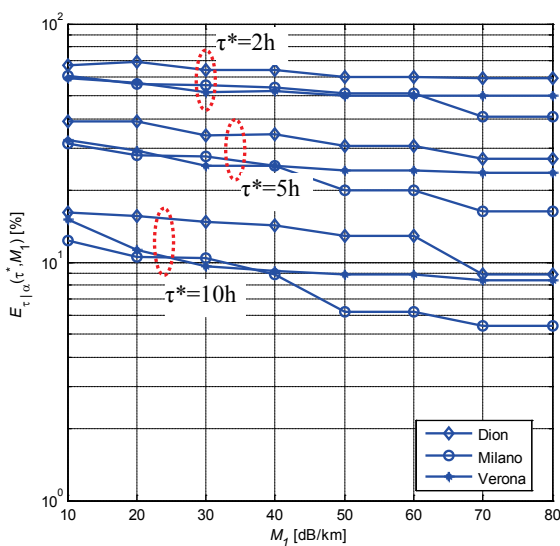
Fig. 5 Conditional probability for selected \tau^* as function of M_1 .
