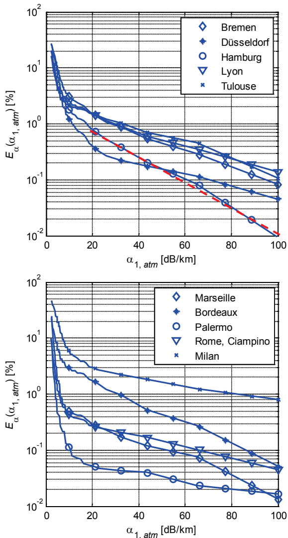
Fig. 3 Empirical E_\alpha for selected sites (approximation- dashed).
