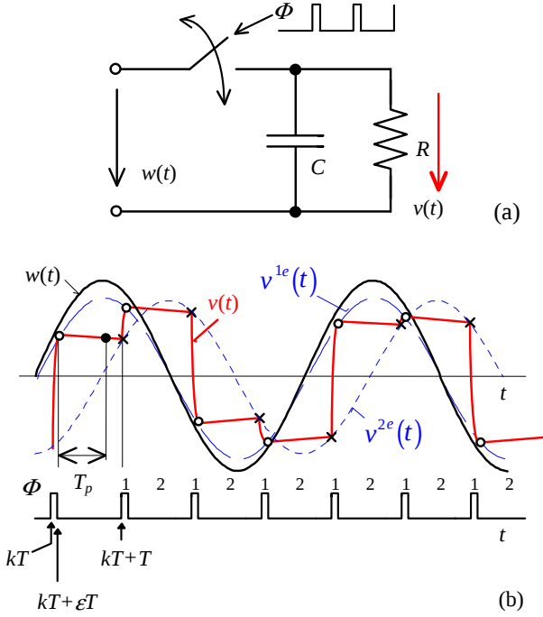
Fig. 1: (a) Model of the Sample-and-Hold circuit, (b) the corresponding waveforms.
