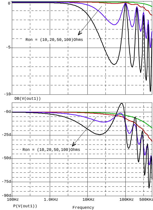
Fig. 2: Amplitude and phase frequency responses of S-H circuit for equivalent signal v^{1e} .
