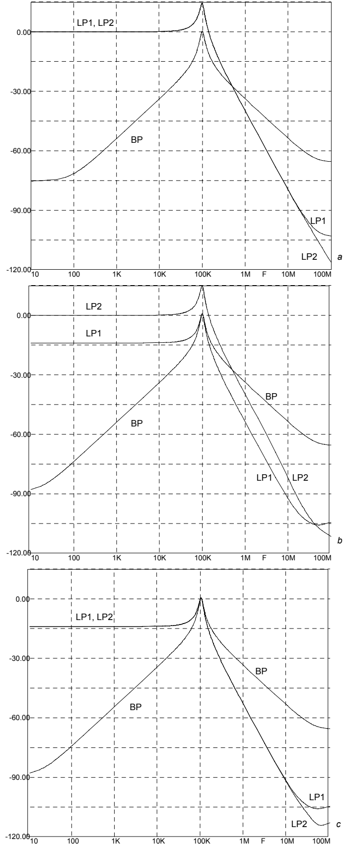
Fig. 6. Frequency responses of the filter from Fig. 1a, a element values according to (3), b lowering the gain peak in LP1 output to the level of BP peak, c lowering the gain peak in LP2 output to the level of BP peak.
