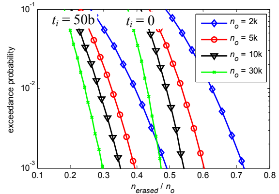
Fig. 8. Effect of block size of outer code ( P_N/N_0 = 8.1dB ).
