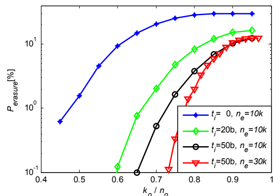
Fig. 9. Probability of packet erasure as function of outer code rate ( P_N/N_0 = 8.1dB , LDGM Triangle, degree 3).
