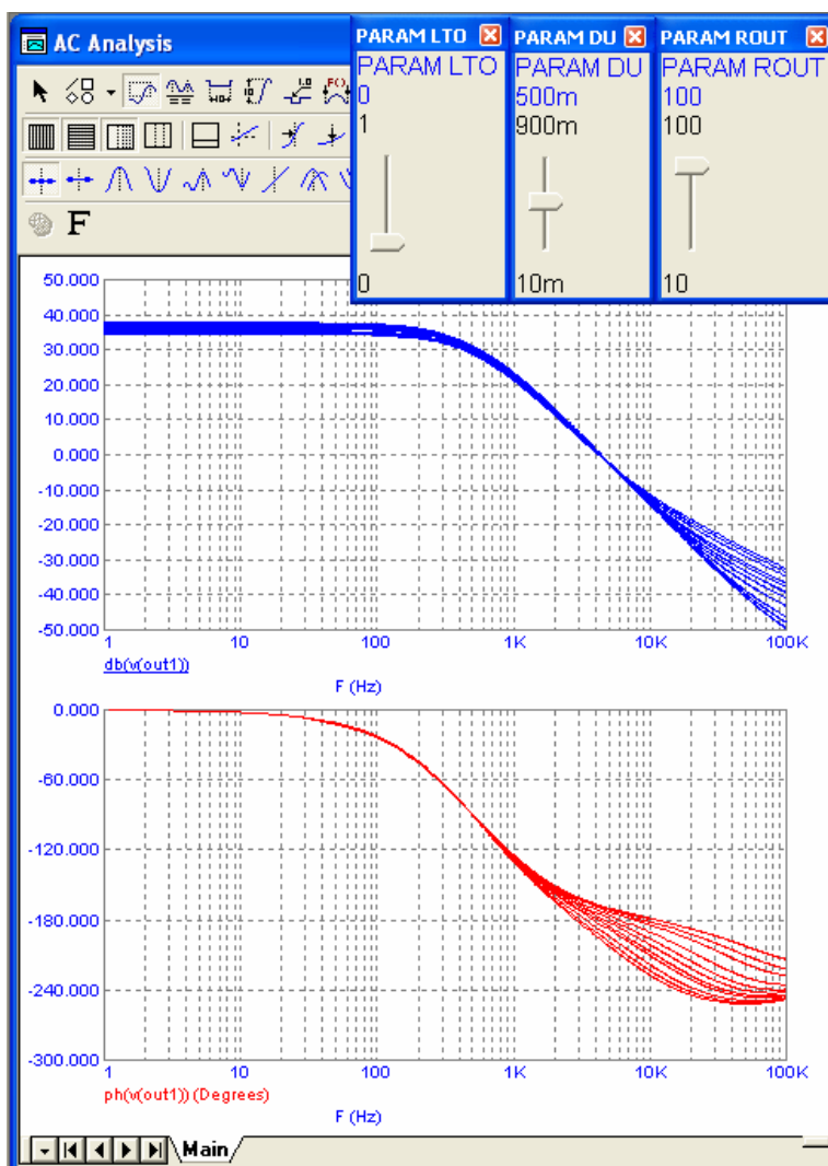
Fig. 4: Demonstration of interactive AC analysis.
