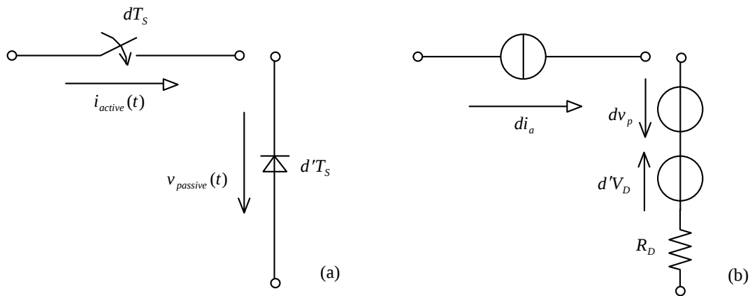
Fig. 1: (a) Pair of active and passive switches, (b) their averaged model. T_s is switching period, d is the duty ration, d'=1-d , V_D is diode forward voltage drop, R_D is diode differential on-resistance [6].
