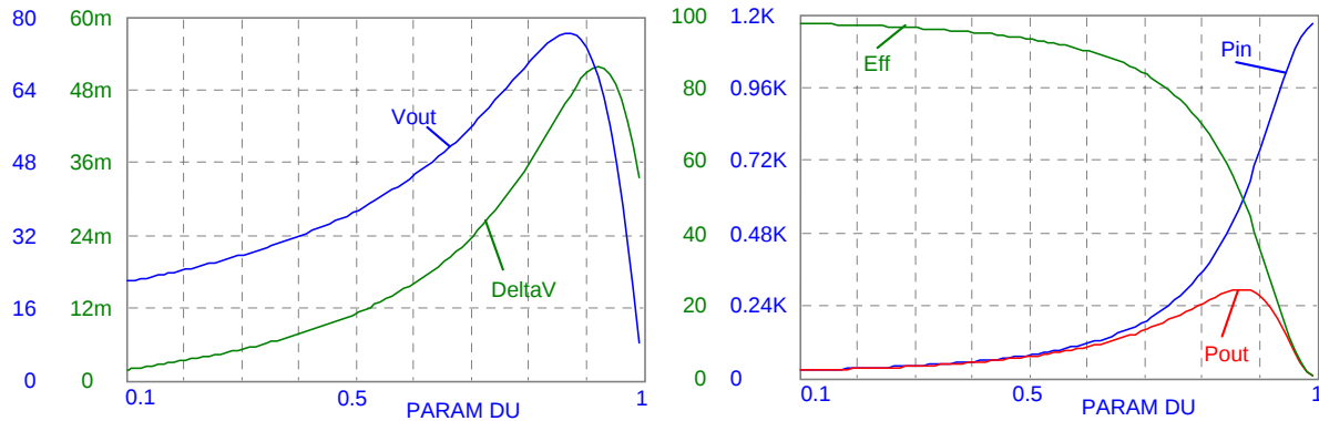
Fig. 4: A demonstration of advanced DC analysis of DC-DC converter.
