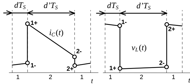
Fig. 2: Piece-wise approximation of time derivatives of converter state variables.
