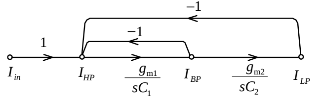
Fig. 1 Flow graph of current-mode KHN biquad
