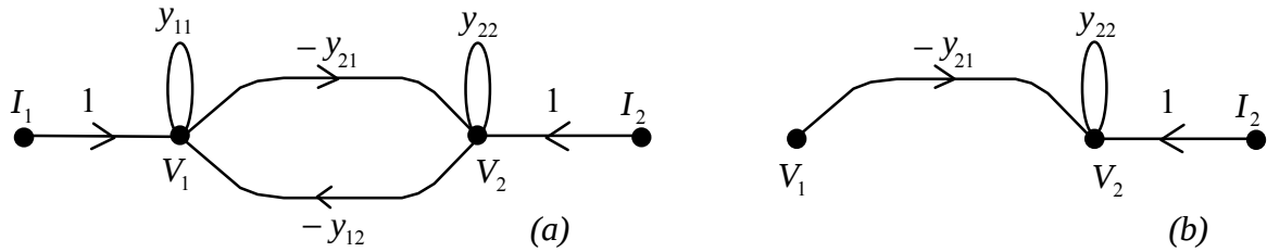
Fig. 1. MC graphs corresponding to the set of equations (1): (a) complete, (b) shortened.
