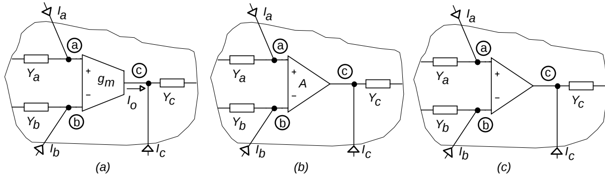
Fig. 2. The OTA (a), ideal voltage amplifier (b) and OPA (c) elements, incorporated in a general circuit.
