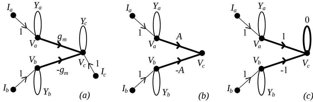
Fig. 3. MC graphs of circuits in Fig. 2.
