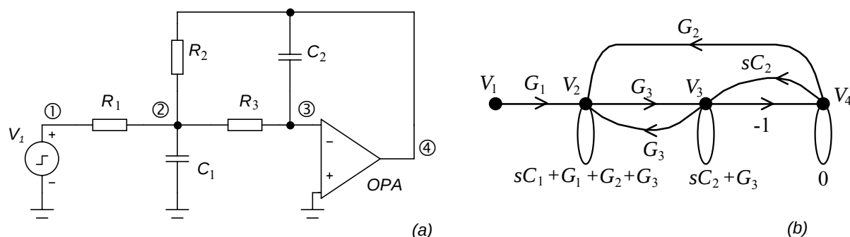
Fig. 4. (a) 2 nd -order filter, (b) the corresponding MC graph.
