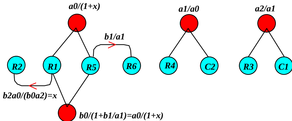
Fig. 15. Graph after the fourth simplifying step.
