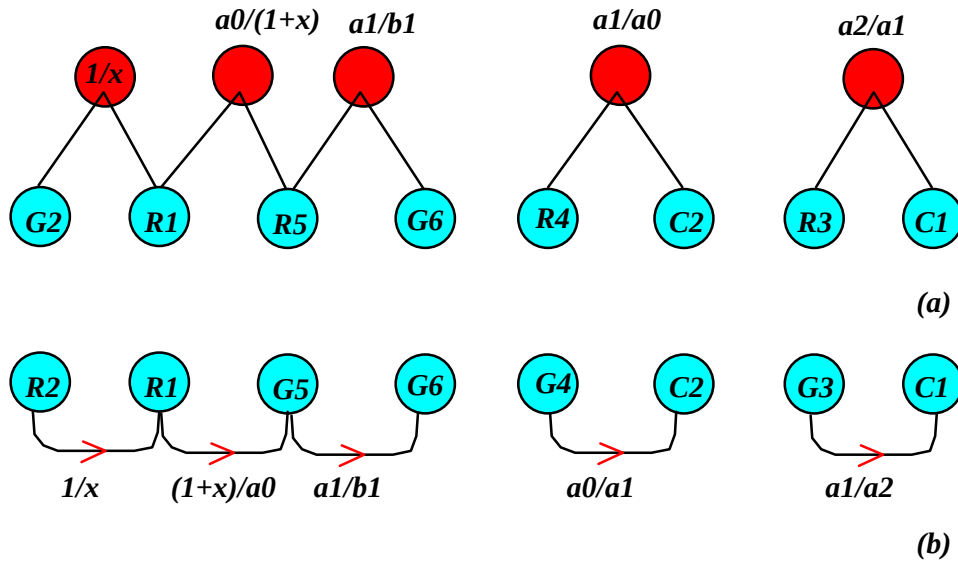
Fig. 16. Graph after the fifth simplifying step, (a) VERTEX, (b) causal.
