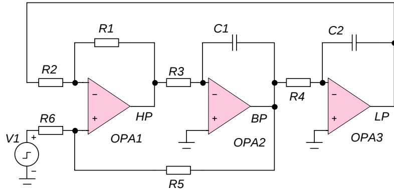
Fig. 10. Example of the KHN-type filter [3].
