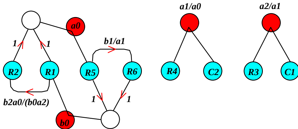
Fig. 14. Graph after the third simplifying step.
