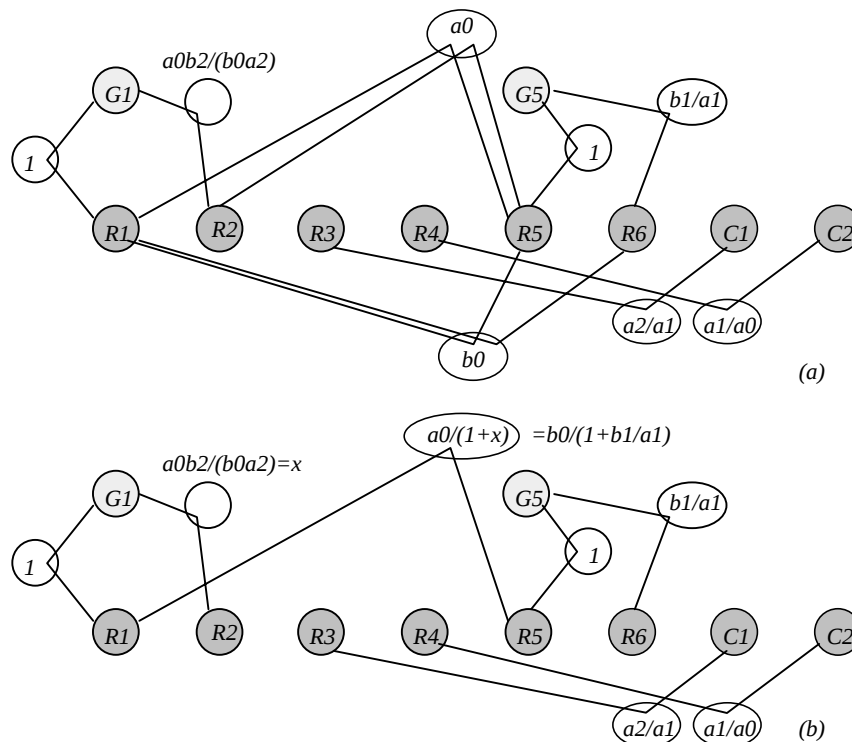
Fig. 4. Vertex graph of the active filter in Fig. 3, (a) initial, (b) minimum.
