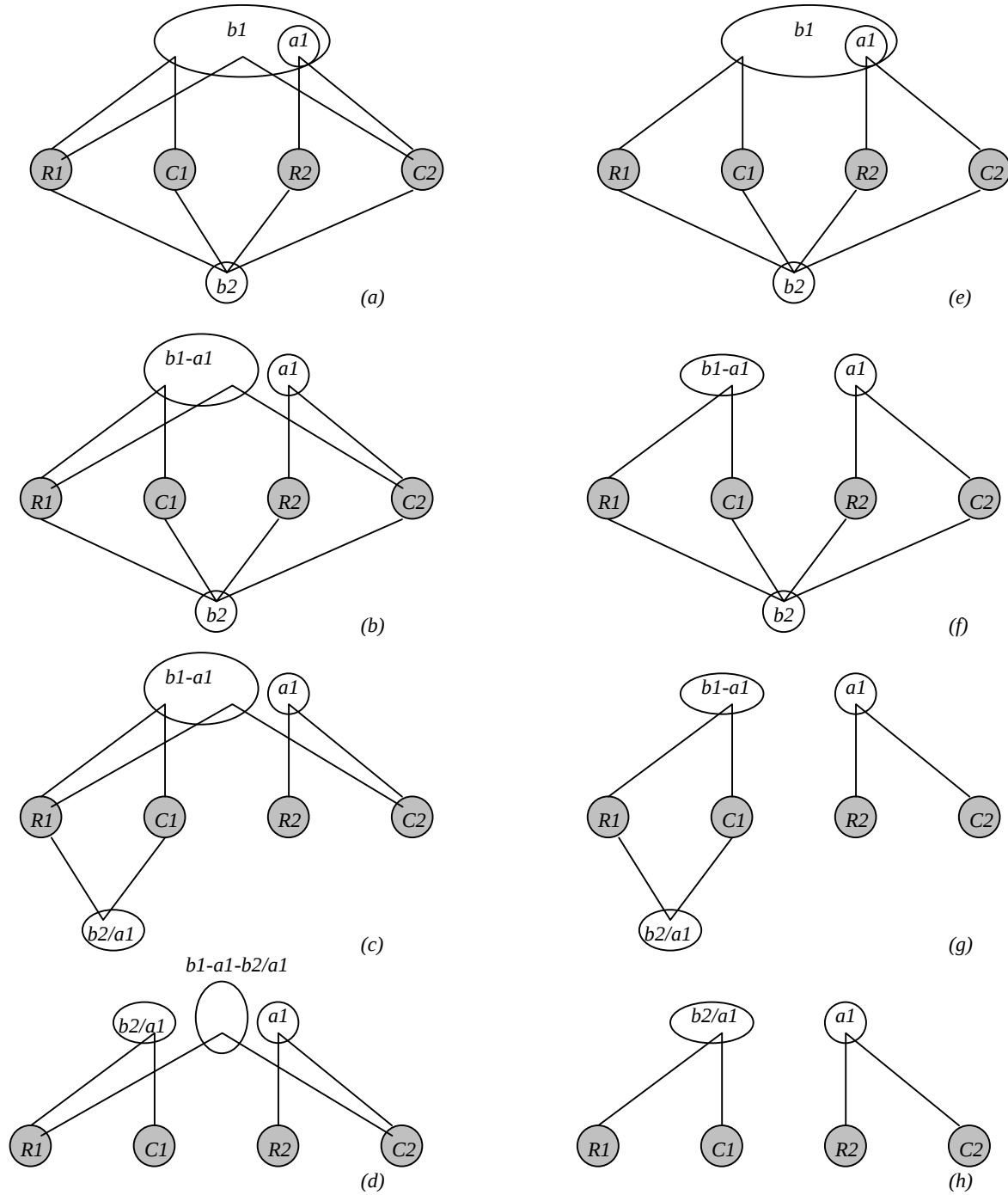
Fig. 2. Coupling graph of the circuit in Fig. 1 and its successive simplification: (a)-(d) full, (e)-(h) reduced after neglecting „weak“ couplings. It holds: b1-a1=R1C1+R1C2 (full graph), or R1C1 (reduced); b2/a1=R1C1 ; b1-a1-b2/a1=R1C2 (full graph), or 0 (reduced).
