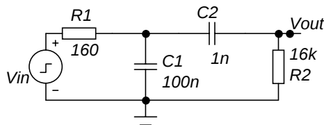
Fig. 1. Example of a passive RC bandpass filter with f_0=10kHz .
