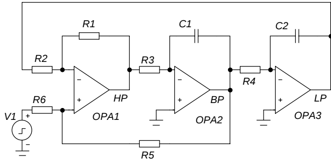
Fig. 3. Active KHN filter [2].
