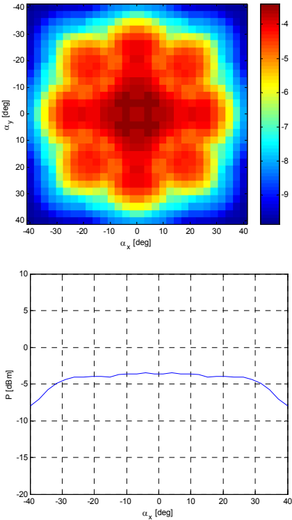
Fig. 4 Distribution of transmitter field received by 15mm test aperture.
