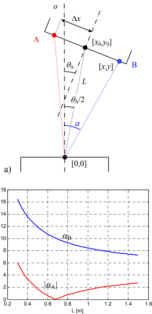
Fig. 1 Simplified geometrical model for determination of \alpha_A and \alpha_B ( \theta_A – angular divergence of wagon axes; \alpha – angular position of opposite device with respect to the optical axis o ; L – distance between [0,0] and [x_0, y_0] ).
