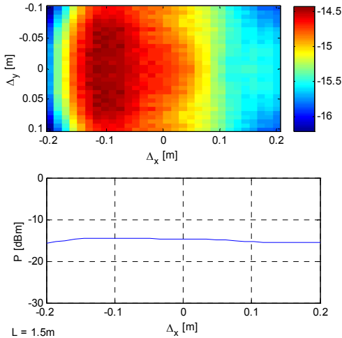
Fig. 5 Received power as function of \Delta x and \Delta y (see Fig.1)
