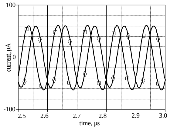
Fig. 3: PSPICE simulation results: steady-state oscillation, \square I_{out1} , \diamond I_{out2} .
