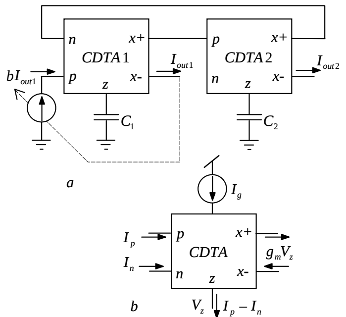
Fig. 1: Proposed QO circuit employing CDTA elements, a) circuit diagram indicating a possibility of gain control, b) CDTA symbol.
