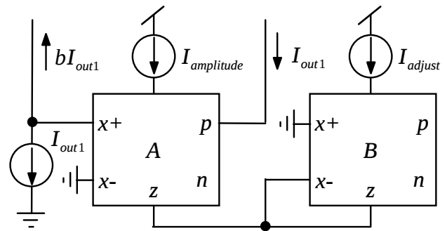
Fig. 2: Proposed circuit for automatic gain control.
